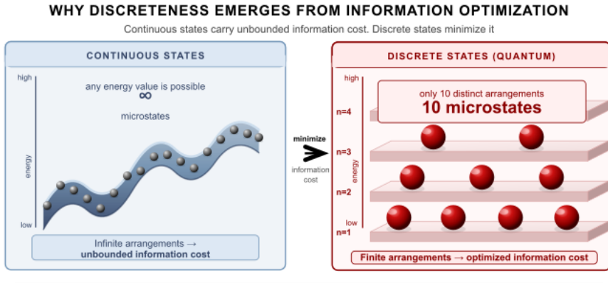
Figure 9 - 1 Continuous systems carry an unbounded information cost; discrete systems minimize it. If physical reality optimizes information storage, discreteness is the predicted outcome, exactly what quantum mechanics shows.
